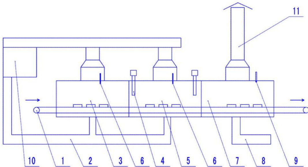
Schematic diagram of LD1504 agricultural and sideline products microwave hot air dehydration drying equipment
